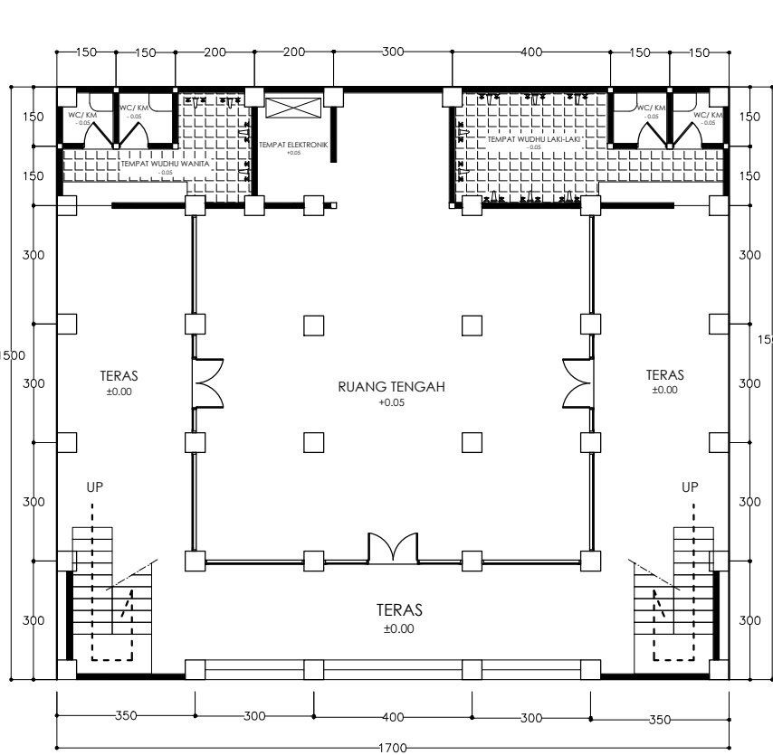
DENAH LT 1 SKALA 1:100
